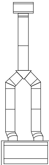
3. Zero Clearance Y Piece - Offset
