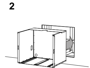
OSK fitted and gas & power services installed
