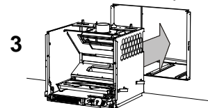
Cavity created and flue installed
