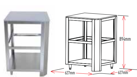
Model: GFK-CN
